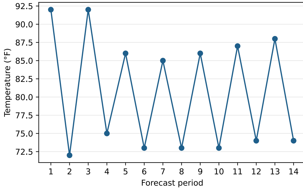
Figure 1: Forecast temperature by period in chronological order
