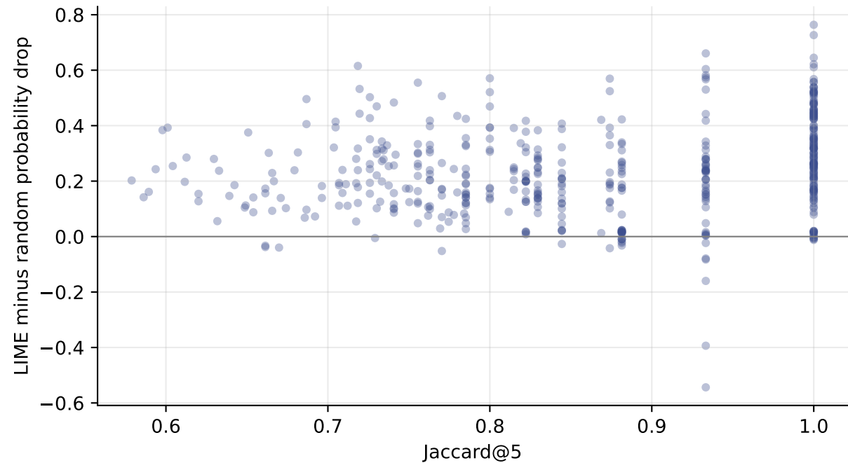
RandomForest: matched historical cases
