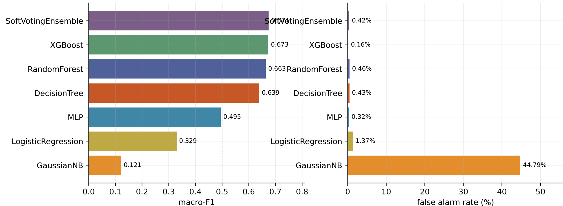
Detection performance (multiclass)
