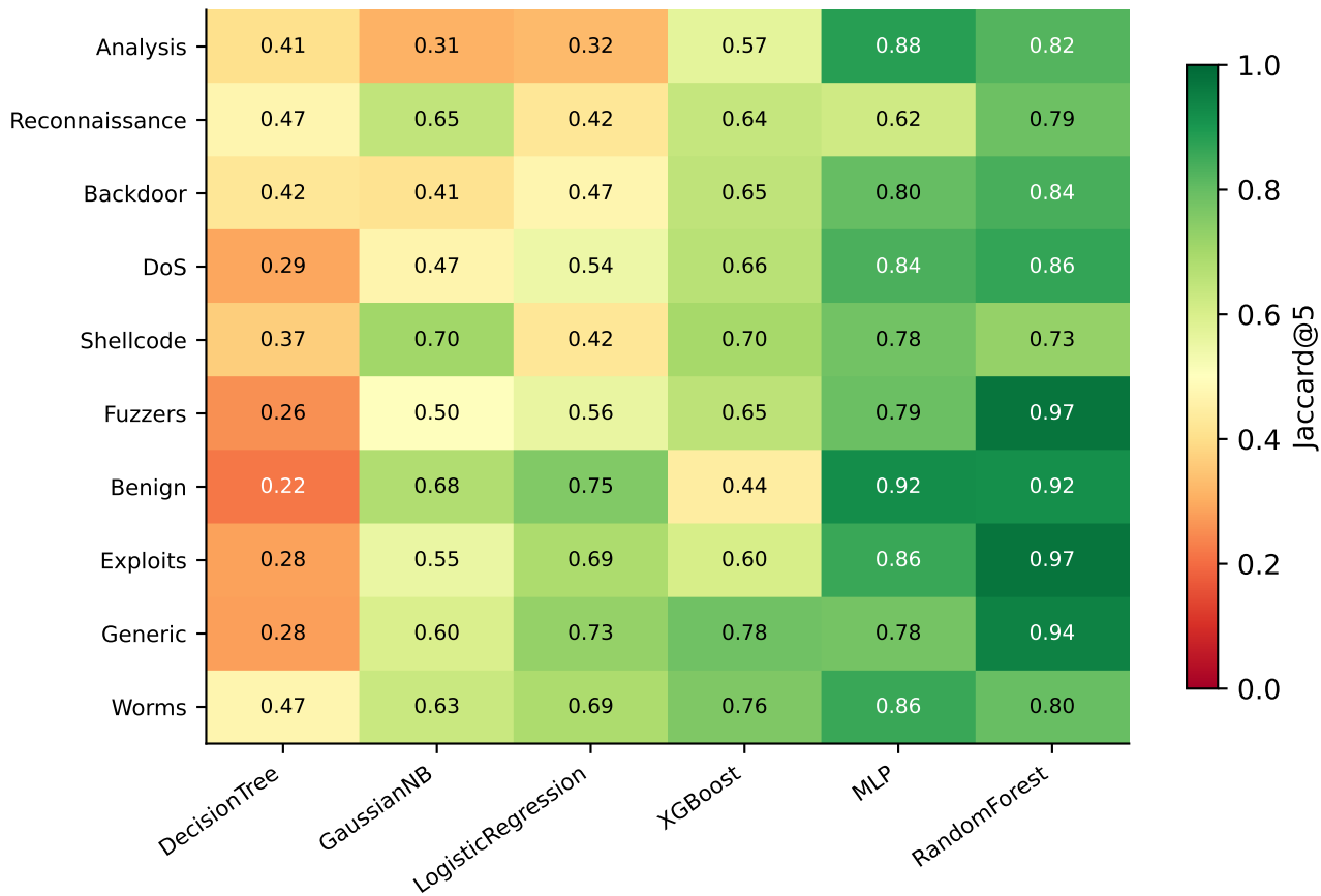
RQ1 — mean Jaccard@5 by attack class and model
