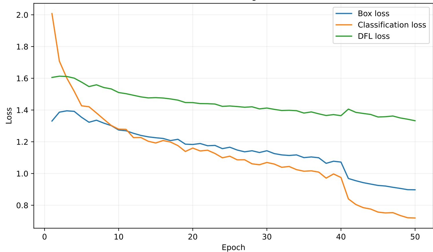
YOLOv8n Training Losses
