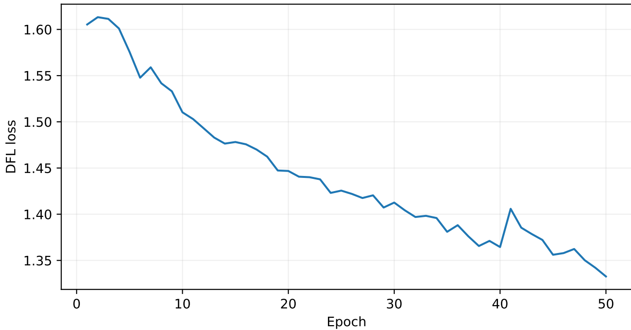
Training Distribution Focal Loss
