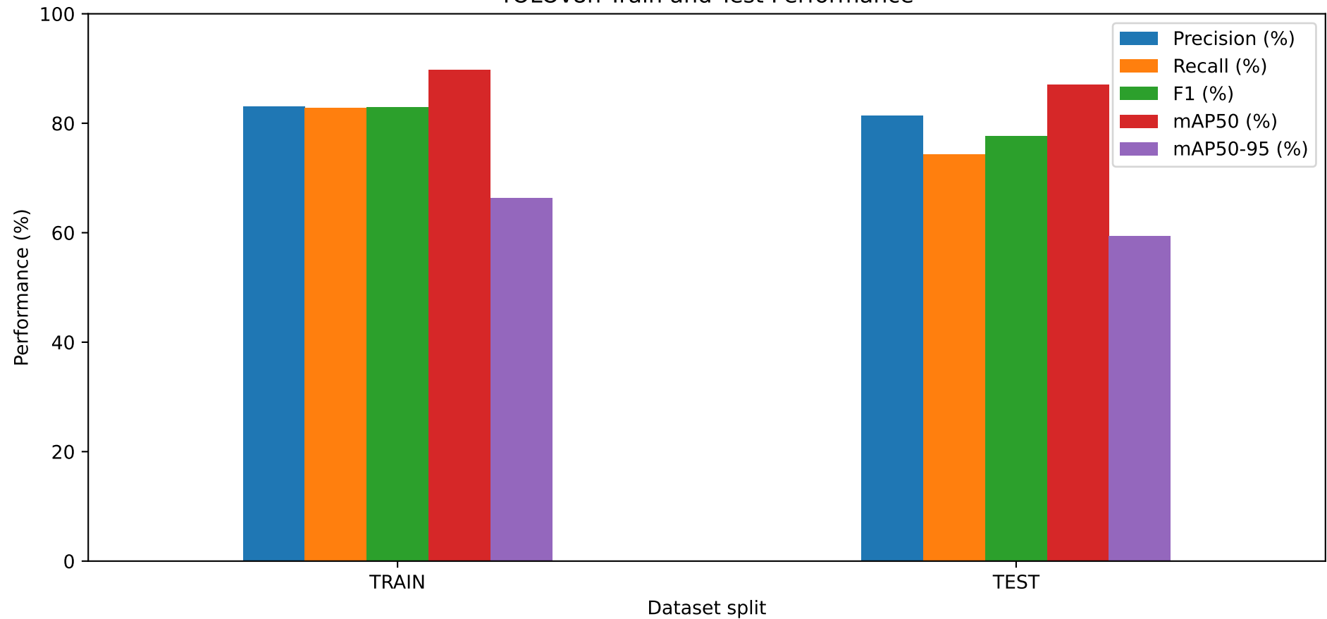
YOLOv8n Train and Test Performance
