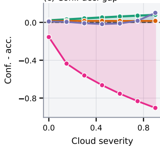
(c) Conf.-acc. gap
