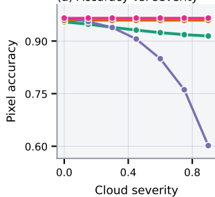
(a) Accuracy vs. severity
