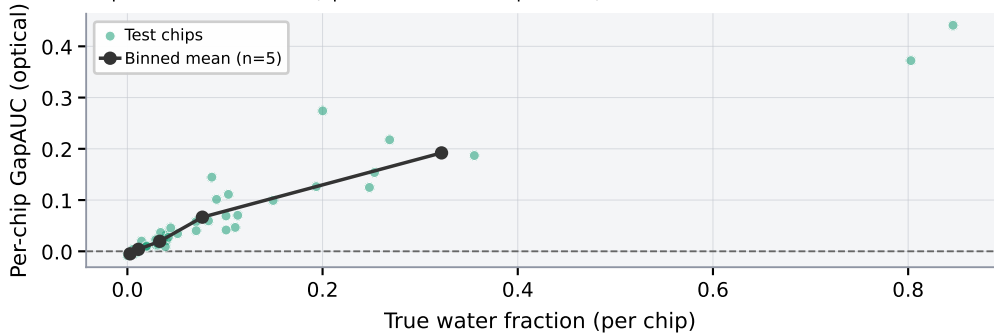
GapAUC vs. flood extent (Spearman rho=0.98, p=0.000)
