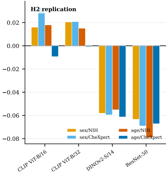
\Delta AUROC vs. BioMedCLIP
