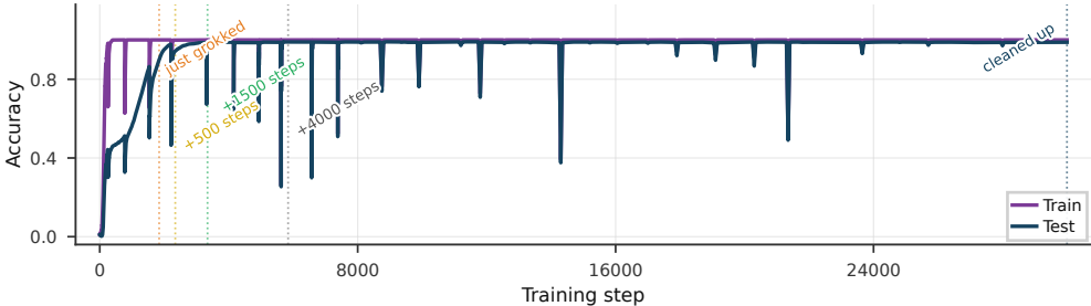
Representative grokking trajectory and checkpoints
