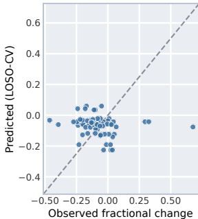
(b) Predictor fit on its own evidence: R^2=-0.33 , MAE=0.12
