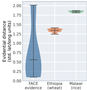
(a) Distance to the real FACE evidence base
