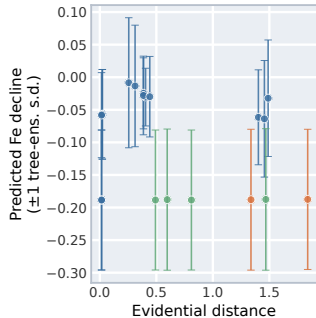
(c) Uncertainty tracks distance weakly ( r=0.33 )
