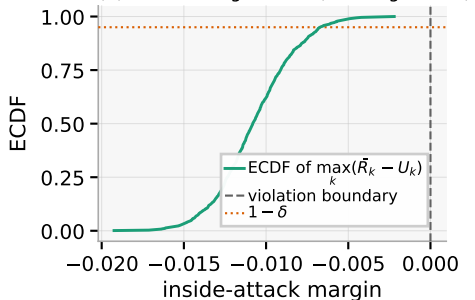
(b) Attack-margin ECDF (all margins < 0)
