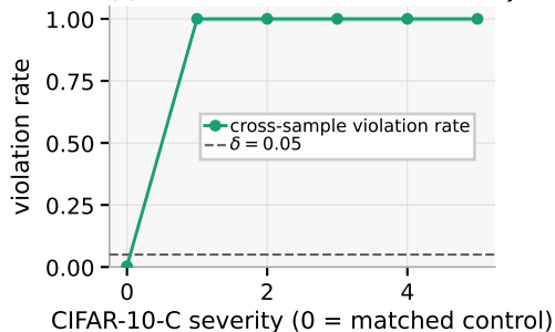
(a) Violation rate vs. CIFAR-10-C severity
