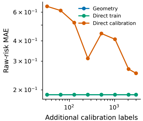
(c) Assessment label budget
