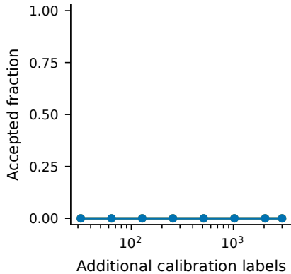
(b) Tolerance = 0.02
