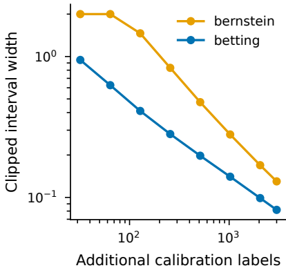
(a) Interval width
