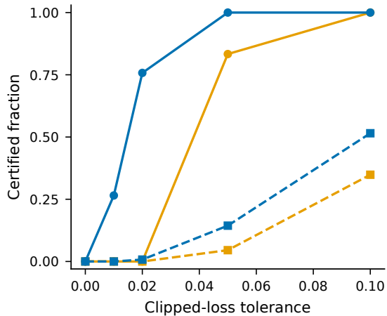
(b) Bounded decision utility
