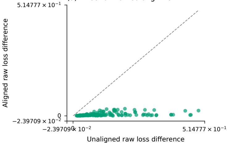
(a) Effect of trained alignment
