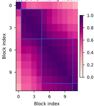
(a) CKA similarity matrix
