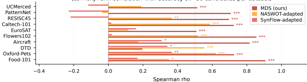
(a) Proxy rank-correlation with accuracy (N=50 candidates per dataset)
