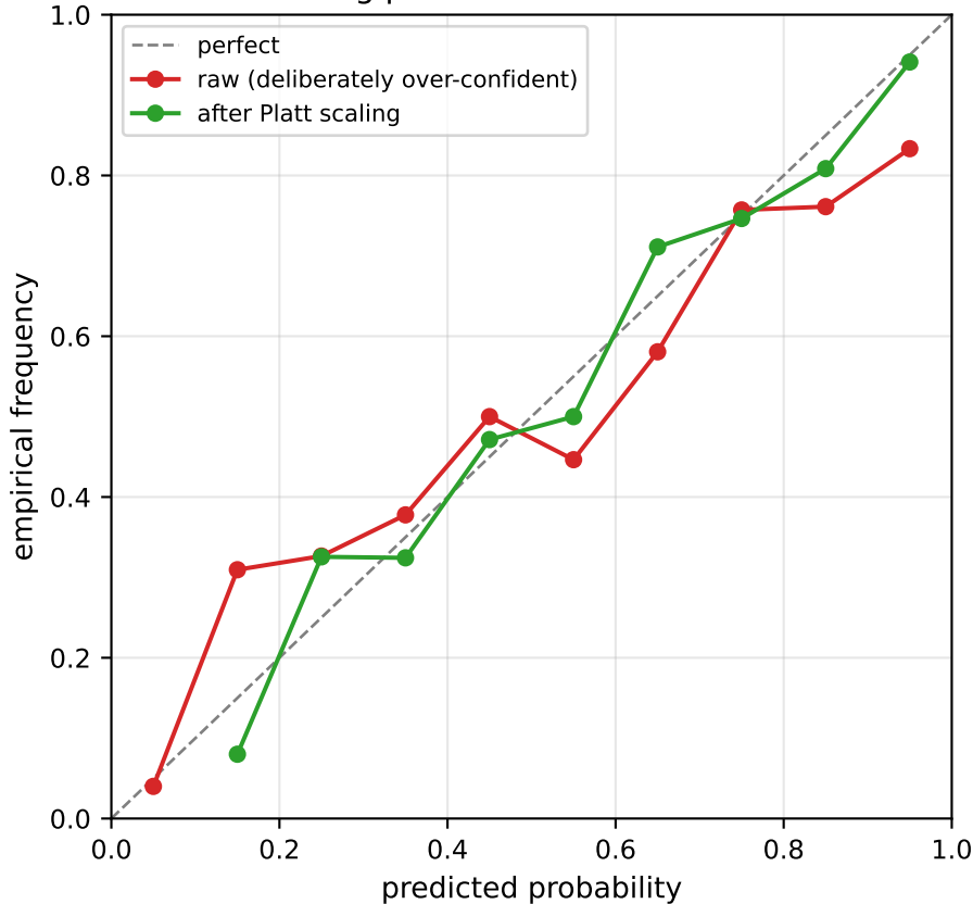
Calibration: Platt scaling pulls a miscalibrated model to the diagonal
