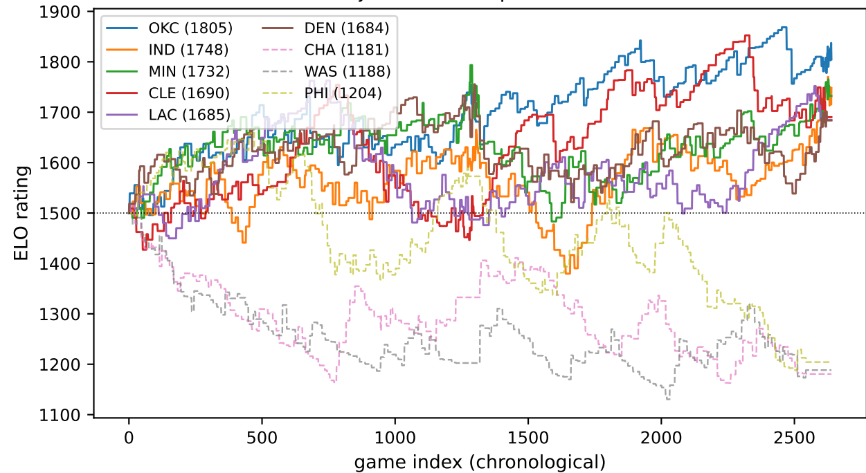
ELO trajectories — top 6 and bottom 3
