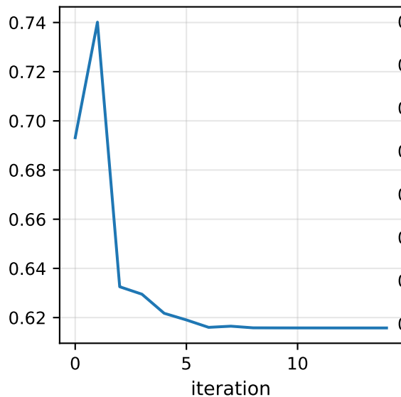
L-BFGS (superlinear)
