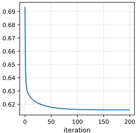
Gradient Descent (linear)
