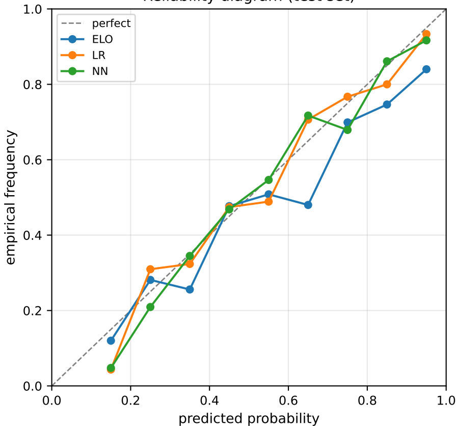
Reliability diagram (test set)
