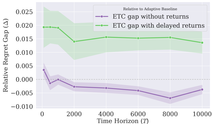
Figure EC.7 Relative-regret gap of ETC with respect to the appropriate adaptive baseline, with and without delayed returns. The purple curve shows \Delta_{\text{no-ret}} , and the green curve shows \Delta_{\text{ret}} . Shaded regions represent standard errors.
