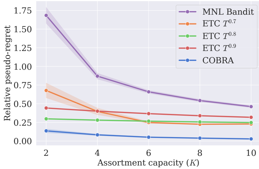
Figure EC.8 Relative regret as a function of the assortment capacity K . As K increases, the capacity constraint becomes less binding and the problem becomes easier for all methods. COBRA remains the best-performing policy throughout.
