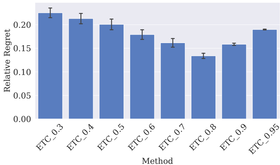
Figure EC.5 The performance of ETC algorithms with respect to various exploration durations controlled by \zeta variable.
