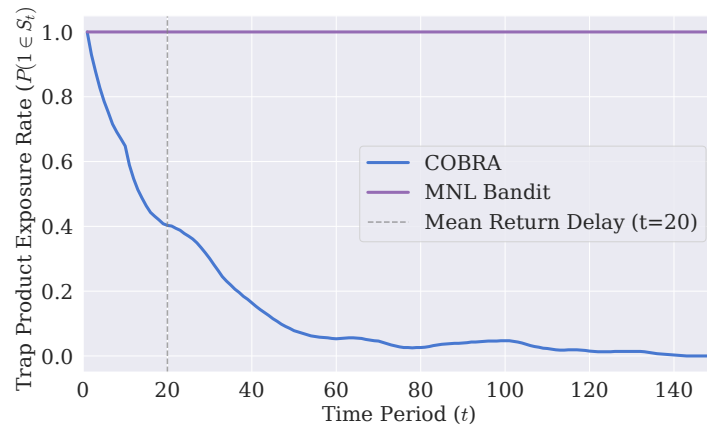
Figure EC.6 Exposure rate of the trap product over time. The dashed vertical line marks the mean return delay. MNL-Bandit keeps the trap product in the assortment throughout, whereas COBRA reduces exposure steadily and drives it close to zero after learning the delayed return signal.
