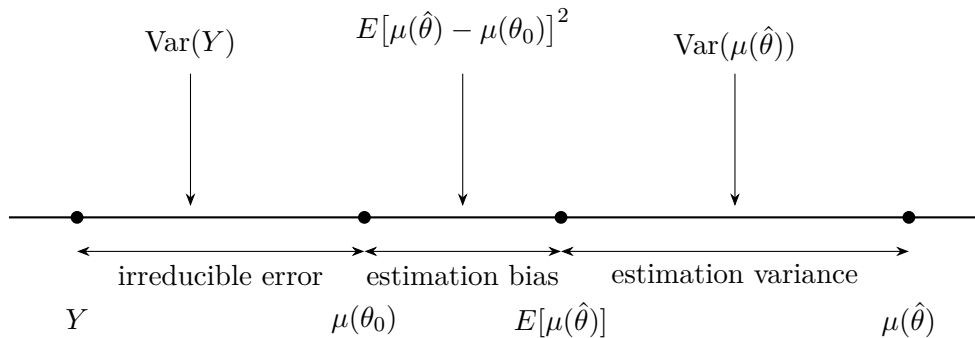
Figure 1.1: Bias-variance decomposition on the number line: the estimand Y , the true conditional mean \mu(\theta_0) , the average fitted value E[\mu(\hat{\theta})] , and a fitted value \mu(\hat{\theta}) .
