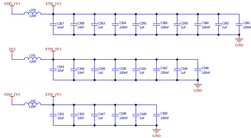
Ethernet Decoupling Capacitors
