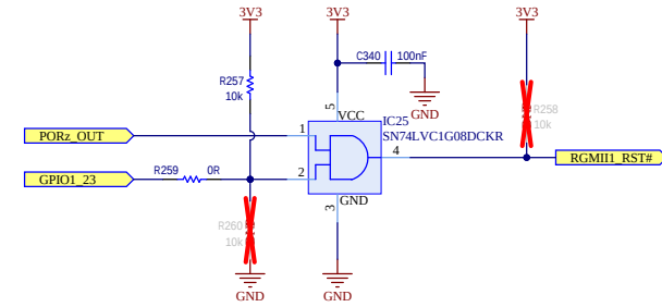
Ethernet AND Gate
