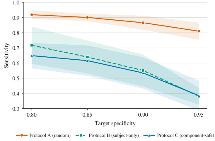
Fig. 10: Sensitivity against target specificity on ADNI1, mean over five seeds with \pm 1 SD bands. The leaky protocol’s advantage is not an artefact of the 0.90 anchor: it holds across the sweep, and widens as the operating point tightens, which is the direction that matters for screening. Protocol B crosses below Protocol C near 0.95, the same inversion the component marginal shows in Figure 7(b); Protocol B’s band is the widest of the three, so the component layer’s apparent advantage over subject-only splitting is not stable to the choice of anchor.
