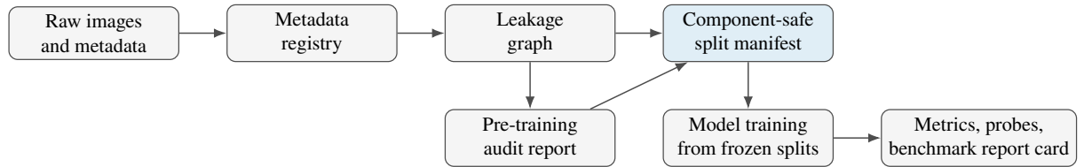
Fig. 2: The SPLITGUARD-AD pipeline: from raw images to audit-verified split manifests and benchmark report cards. Modules are executed sequentially; each produces a versioned artefact consumed by the next.
