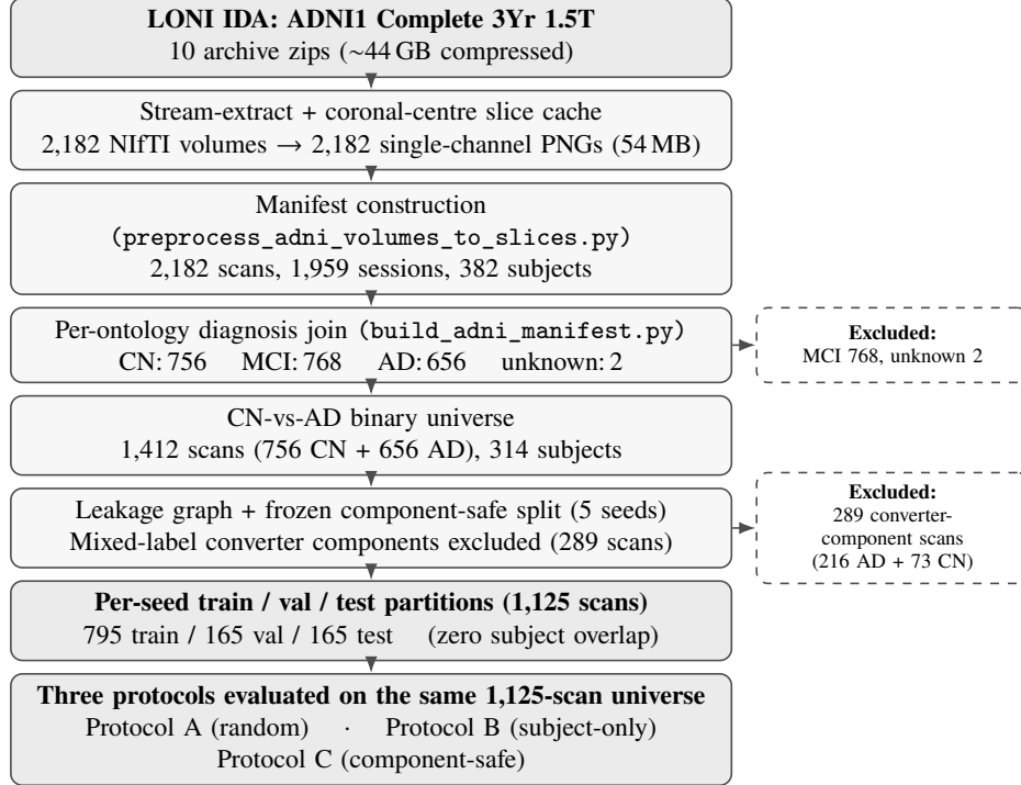
Fig. 3: ADNI1: Complete 3Yr 1.5T data flow from LONI IDA archive download to per-seed train/validation/test partitions. Each transition annotates the row count and the script responsible ( preprocess_adni_volumes_to_slices.py , build_adni_manifest.py , make_adni_splitguard_split.py ). Dashed boxes on the right record exclusions: MCI / unknown diagnoses excluded from the CN-vs-AD task by construction, and 289 CN/AD scans (216 AD + 73 CN) from mixed-label longitudinal converter components excluded from the primary arm and re-included in the sensitivity arm (§3.3).
