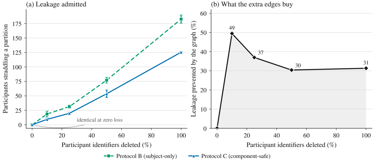
Fig. 10: Provenance degradation on the ADNI1 primary arm, five seeds, mean \pm SD. (a) Participants whose scans straddle a partition boundary as participant identifiers are deleted. This counts admitted leakage directly, without routing the question through a trained model. The two protocols are indistinguishable at zero loss (the equivalence reported in §2.2.2, here the origin of a curve rather than a dead end) and separate immediately thereafter. (b) The share of that leakage the leakage graph prevents. Both protocols use the same assigner, so the difference is attributable to the grouping; under a mismatched assigner the 10% figure reads 78%. The benefit peaks in the regime where redistributed benchmarks sit and decays once too few identifiers survive for any rule to bind on.
