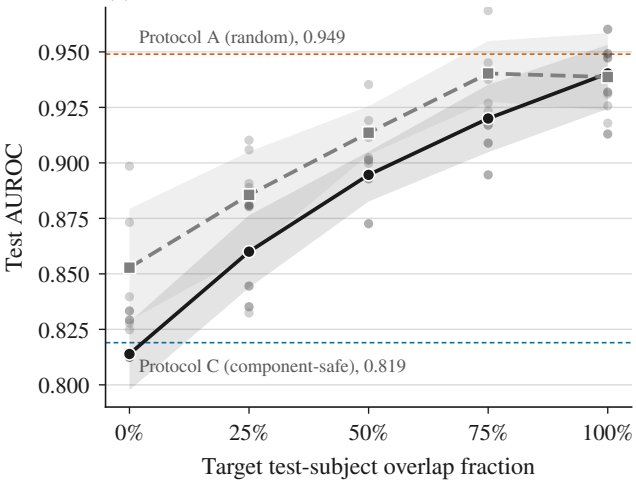
(a) Per-seed AUROC, mean \pm 95% CI
