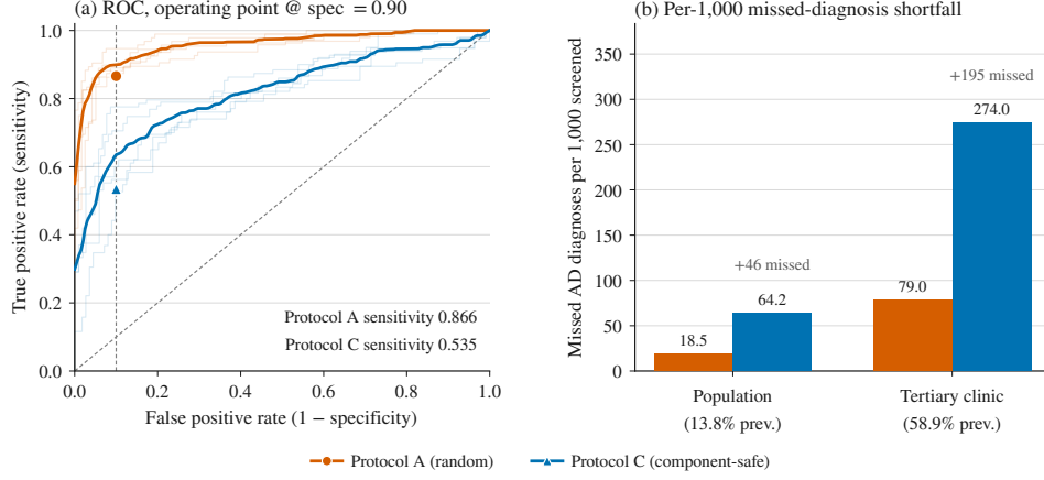
Fig. 9: Arithmetic cost-of-leakage translation on the converter-inclusive ADNI sensitivity arm. (a) Per-seed ROC curves for Protocol A (leaky) and Protocol C (component-safe SPLITGUARD-AD); the dashed vertical line marks the screening operating point at specificity = 0.90 (i.e. false-positive rate = 0.10); markers show the per-seed mean sensitivity at that specificity. (b) Missed AD diagnoses per 1,000 screened patients at the two literature-cited prevalence anchors, computed as 1,000 \cdot \text{prev} \cdot (1 - \text{sens}) . Protocol A’s bars use its apparent sensitivity (0.866) and Protocol C’s bars its honest sensitivity (0.535). The annotation “+ N missed” is the per-1,000 arithmetic shortfall implied by reporting the leaky number instead of the honest one;
