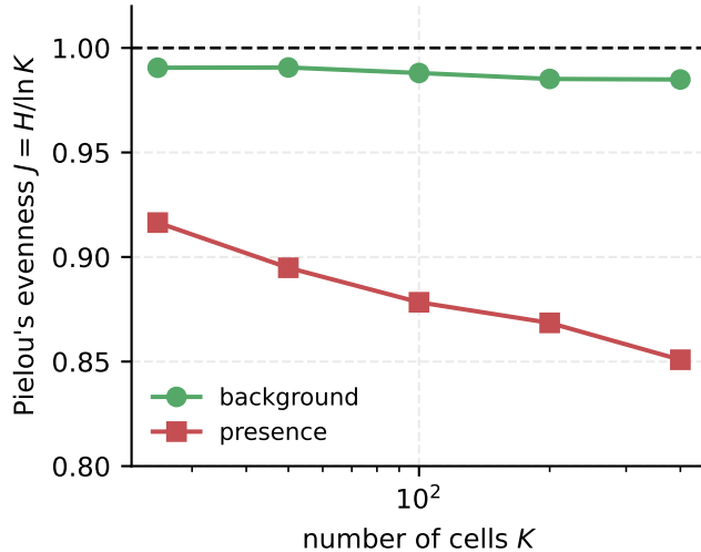
(b) Evenness
