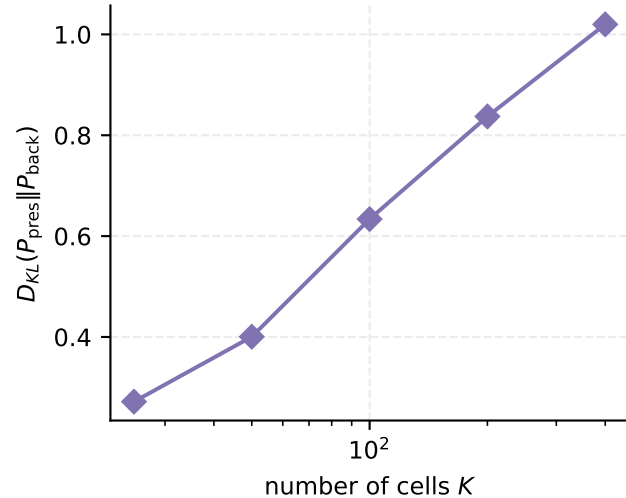
(c) Divergence
