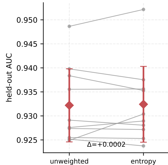
Random Forest
