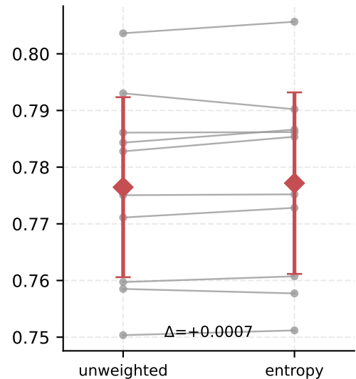
Bayesian
