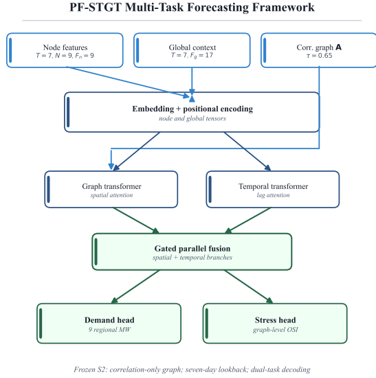
Fig. 1. End-to-end PF-STGT multi-task forecasting framework (frozen S2). Seven-day node and global tensors, a train-estimated correlation graph, parallel spatial-temporal encoding, and dual demand/OSI decoding heads.
