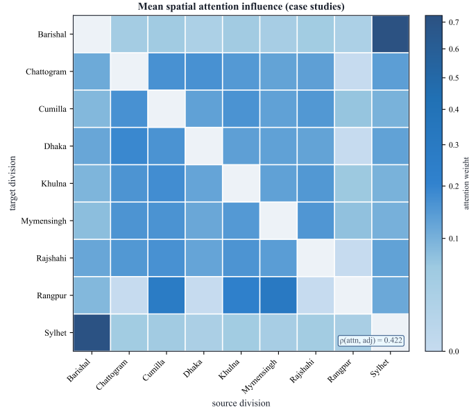
Fig. 3. Mean spatial attention influence on the correlation graph, averaged over 24 case studies. Cell (i, j) gives attention from source division j to target i ; diagonal entries are masked. \rho(\text{attention}, \text{adjacency})=0.422 .
