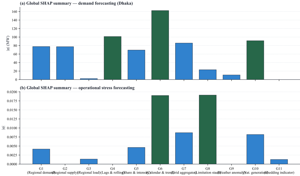
Fig. 4. Grouped GradientSHAP mean absolute attributions ( |\phi| ) on coalition registry G1–G11 (validation n=20 ). (a) Dhaka demand: calendar (G6), lags (G4), and national generation (G10) dominate. (b) Stress: limitation stack (G8) and calendar (G6) rank highest.
