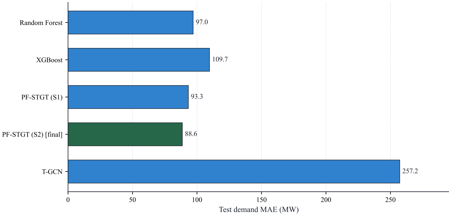
Benchmark comparison — demand forecasting (test set)
