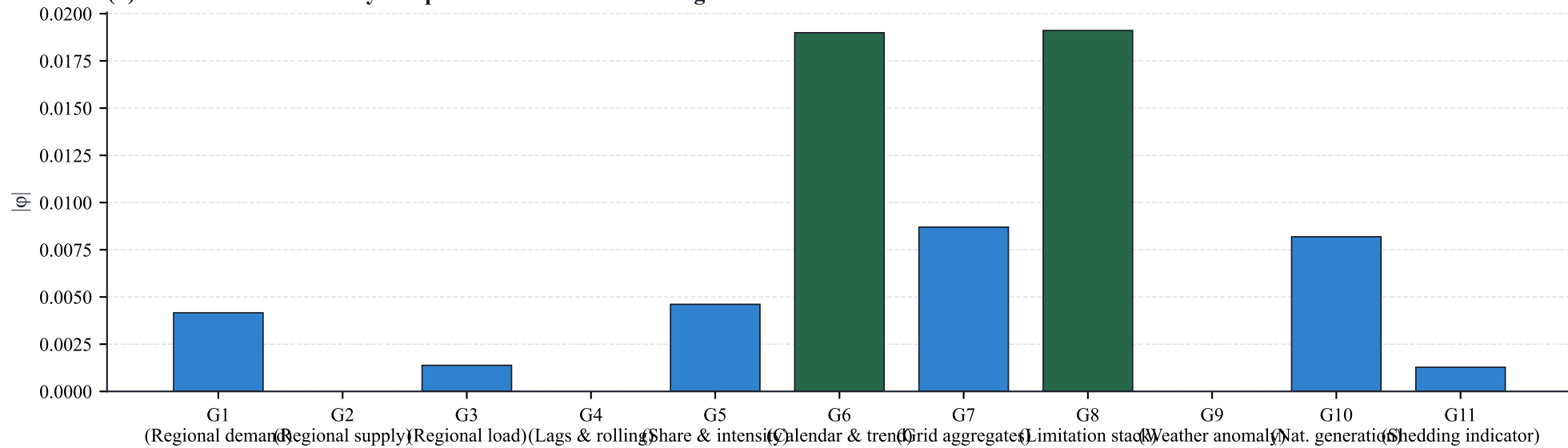
(b) Global SHAP summary — operational stress forecasting
