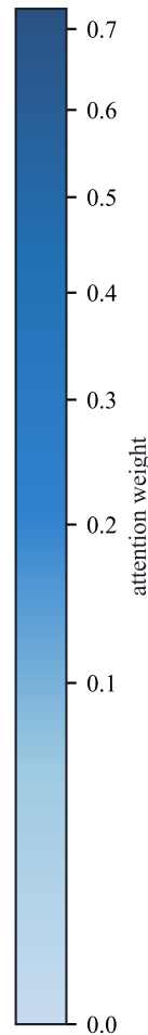
\rho(\text{attn}, \text{adj}) = 0.422
