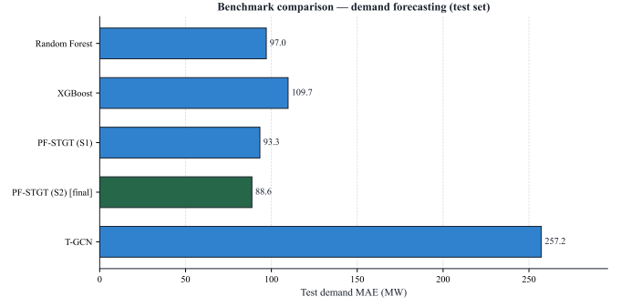
Fig. 4. Test-set macro demand MAE ( n=264 windows). S2 achieves the lowest error (88.65 MW).
