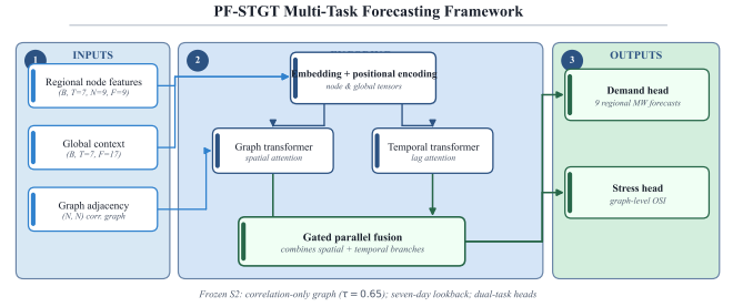
Fig. 1. End-to-end PF-STGT multi-task forecasting framework (frozen S2). Seven-day node and global tensors, a train-estimated correlation graph, parallel spatial-temporal encoding, and dual demand/OSI decoding heads.
