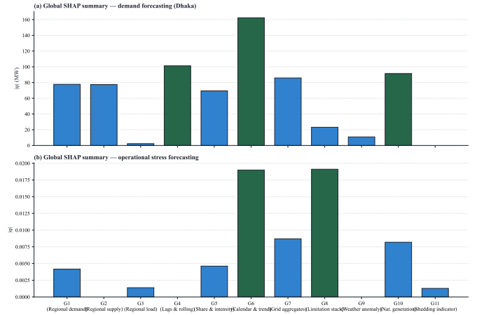
Fig. 6. Grouped GradientSHAP mean absolute attributions ( |\phi| ) on coalition registry G1–G11 (validation n=20 ). (a) Dhaka demand: calendar (G6), lags (G4), and national generation (G10) dominate. (b) Stress: limitation stack (G8) and calendar (G6) rank highest.
