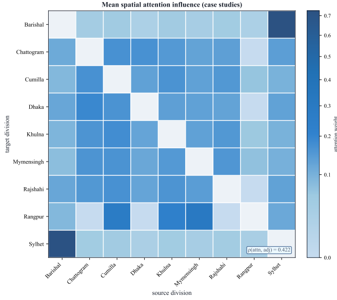
Fig. 7. Mean spatial attention influence on the correlation graph, averaged over 24 case studies. Cell (i, j) gives attention from source division j to target i ; diagonal entries are masked. \rho(\text{attention}, \text{adjacency})=0.422 .
