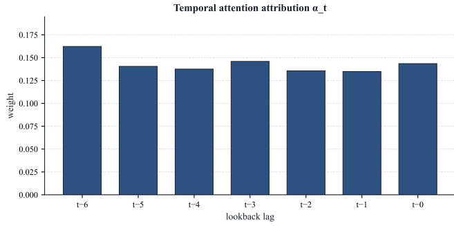
Fig. 8. Mean temporal attention weights \alpha_t across the seven-day input window, averaged over 24 case studies. Weights are near-uniform (peak at t-6 , \alpha=0.1622 ).
