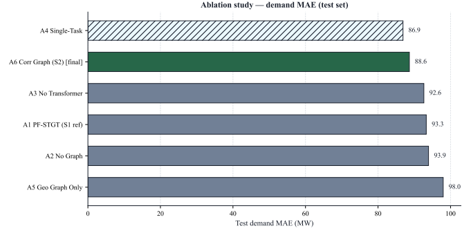
Fig. 5. Ablation demand MAE by configuration on the held-out test split. A4 is demand-only; S2 (A6) leads among multi-task variants.
