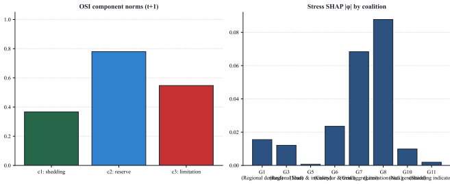
Fig. 9. Dual-path stress attribution on high-stress test day 2024-09-08. Left: normalised OSI component norms at t+1 . Right: grouped stress SHAP |\phi| by coalition; G8 ranks highest.
