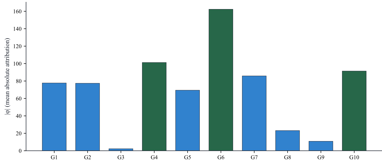
Global demand SHAP — Dhaka ( |\varphi| )
