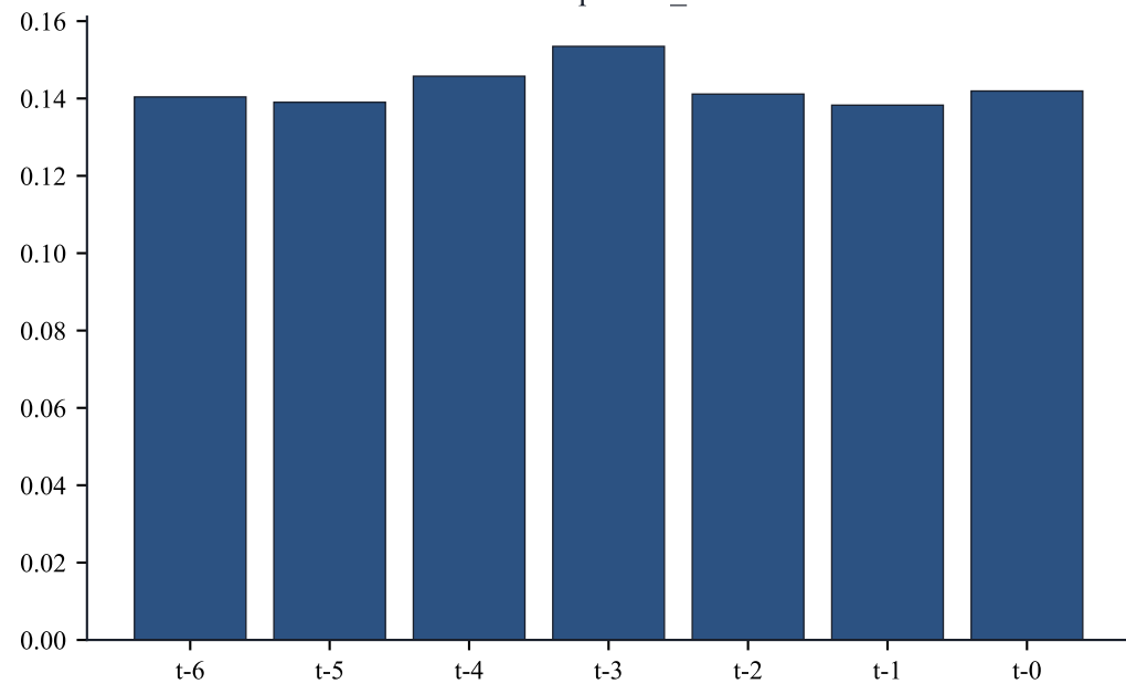
Temporal \alpha_t
