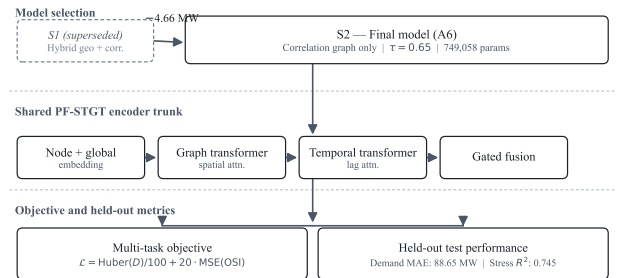
Fig. 2. Frozen S2 (A6) architecture with correlation-only graph ( \tau=0.65 ). S2 replaces hybrid-graph S1 and reports held-out demand MAE of 88.65 MW and stress R^2 of 0.745.
