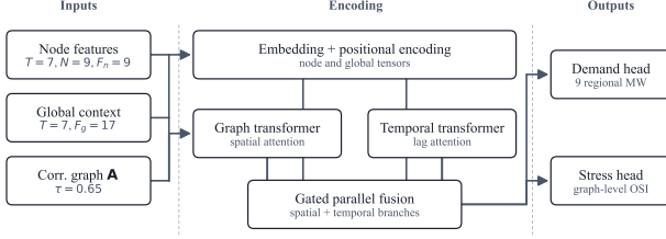
Fig. 1. End-to-end PF-STGT multi-task forecasting framework (frozen S2). Seven-day node and global tensors, a train-estimated correlation graph, parallel spatial-temporal encoding, and dual demand/OSI decoding heads.
