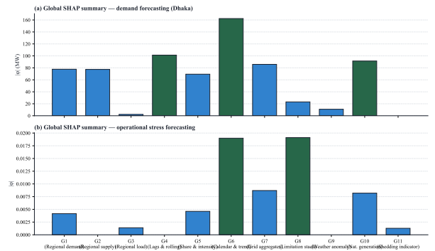
Fig. 6. Grouped GradientSHAP mean absolute attributions ( |\phi| ) on coalition registry G1–G11 (validation n=20 ). (a) Dhaka demand: calendar (G6), lags (G4), and national generation (G10) dominate. (b) Stress: limitation stack (G8) and calendar (G6) rank highest.
