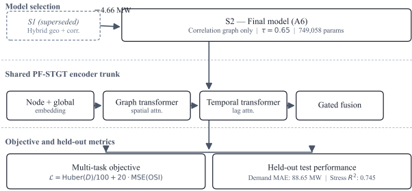
Fig. 2. Frozen S2 (A6) architecture with correlation-only graph ( \tau=0.65 ). S2 replaces hybrid-graph S1 and reports held-out demand MAE of 88.65 MW and stress R^2 of 0.745.
