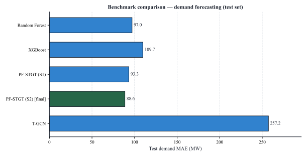
Fig. 3. Test-set macro demand MAE ( n=264 windows). S2 achieves the lowest error (88.65 MW).
