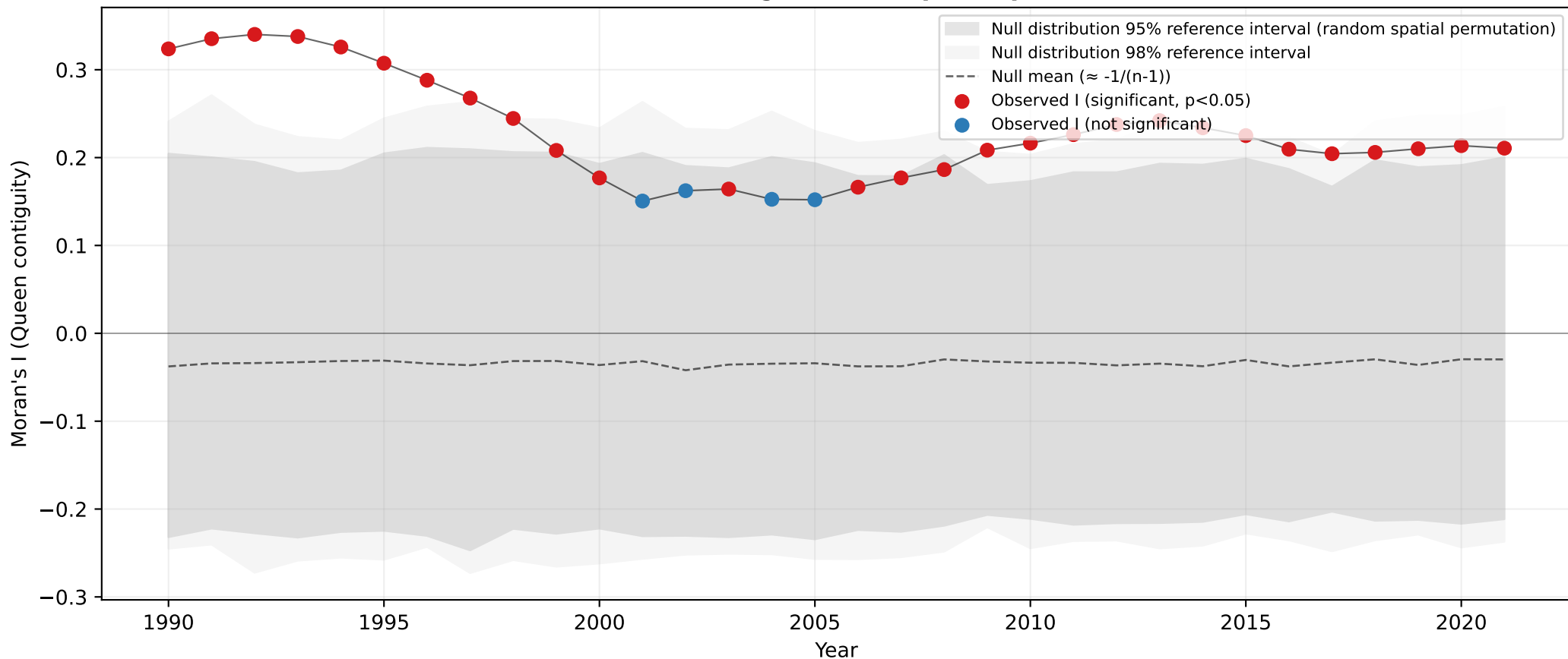
Provincial QCI: observed Moran's I against the spatial-permutation null distribution
