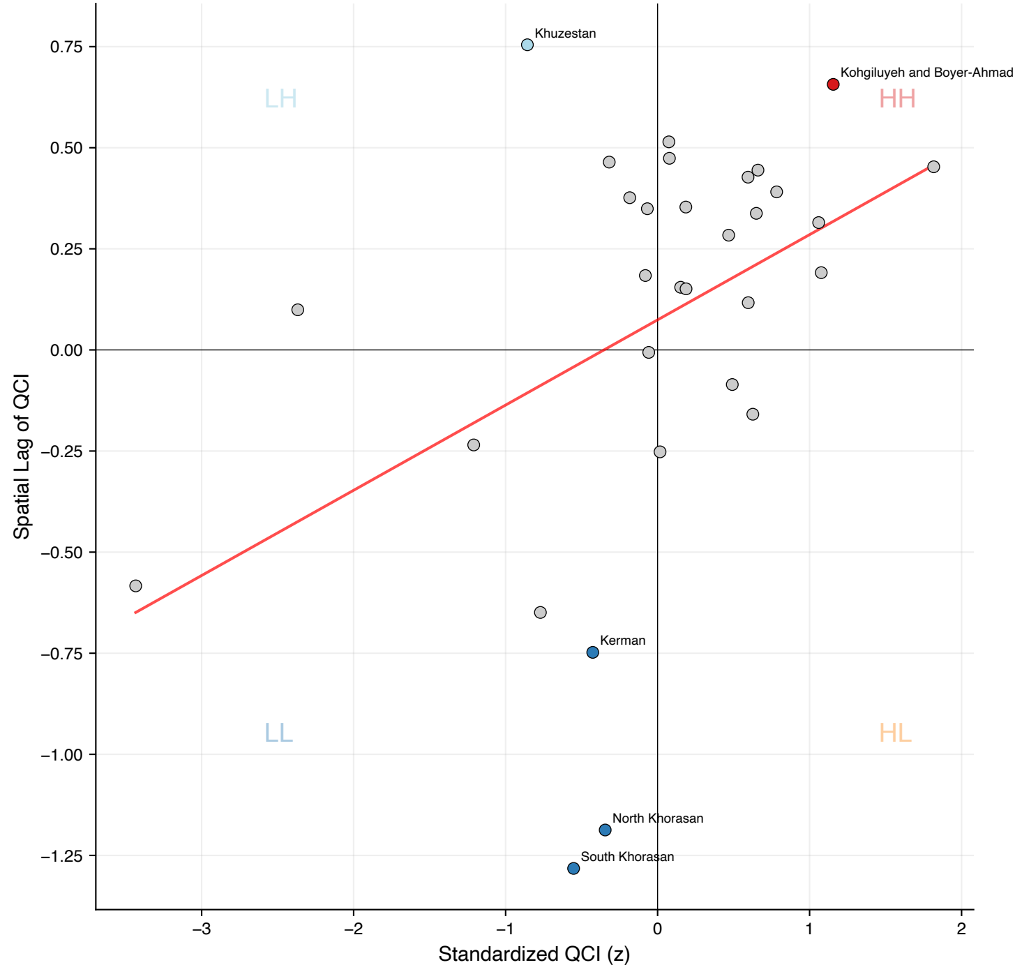
(A) Moran Scatterplot ( I=0.211 , p=0.023 )
