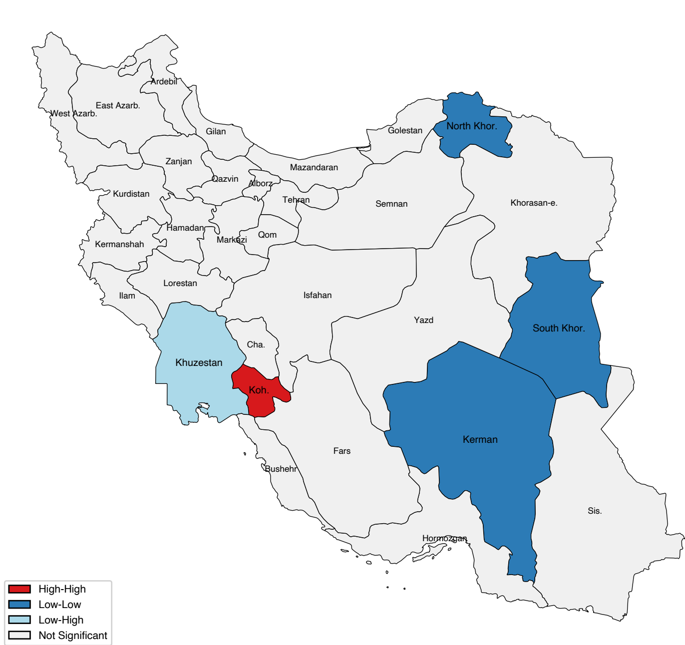
(B) LISA Cluster Map, 2021
