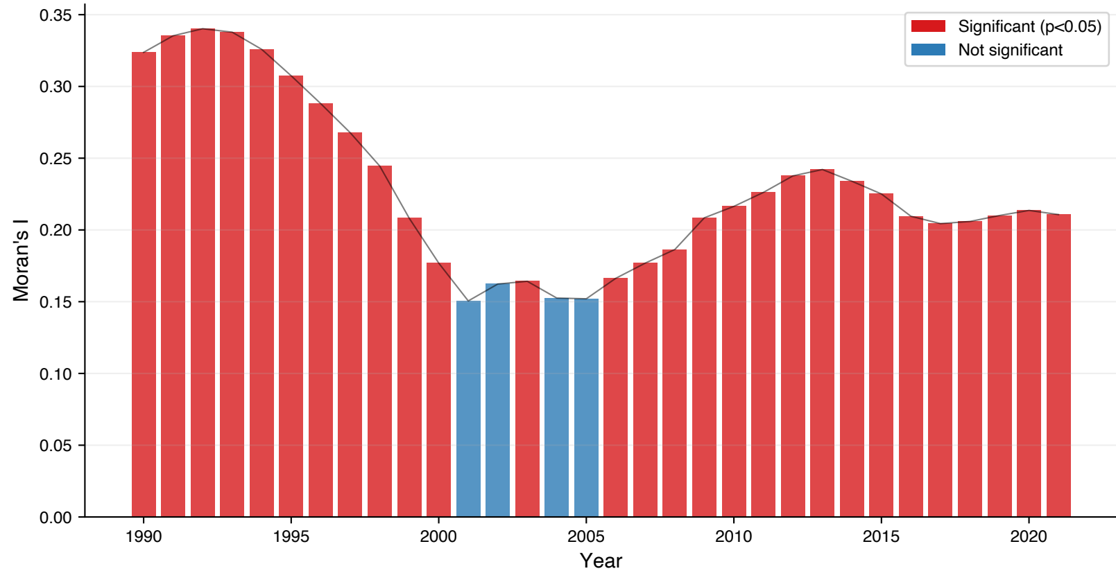
Global Moran's I for Provincial QCI, Iran, 1990-2021
