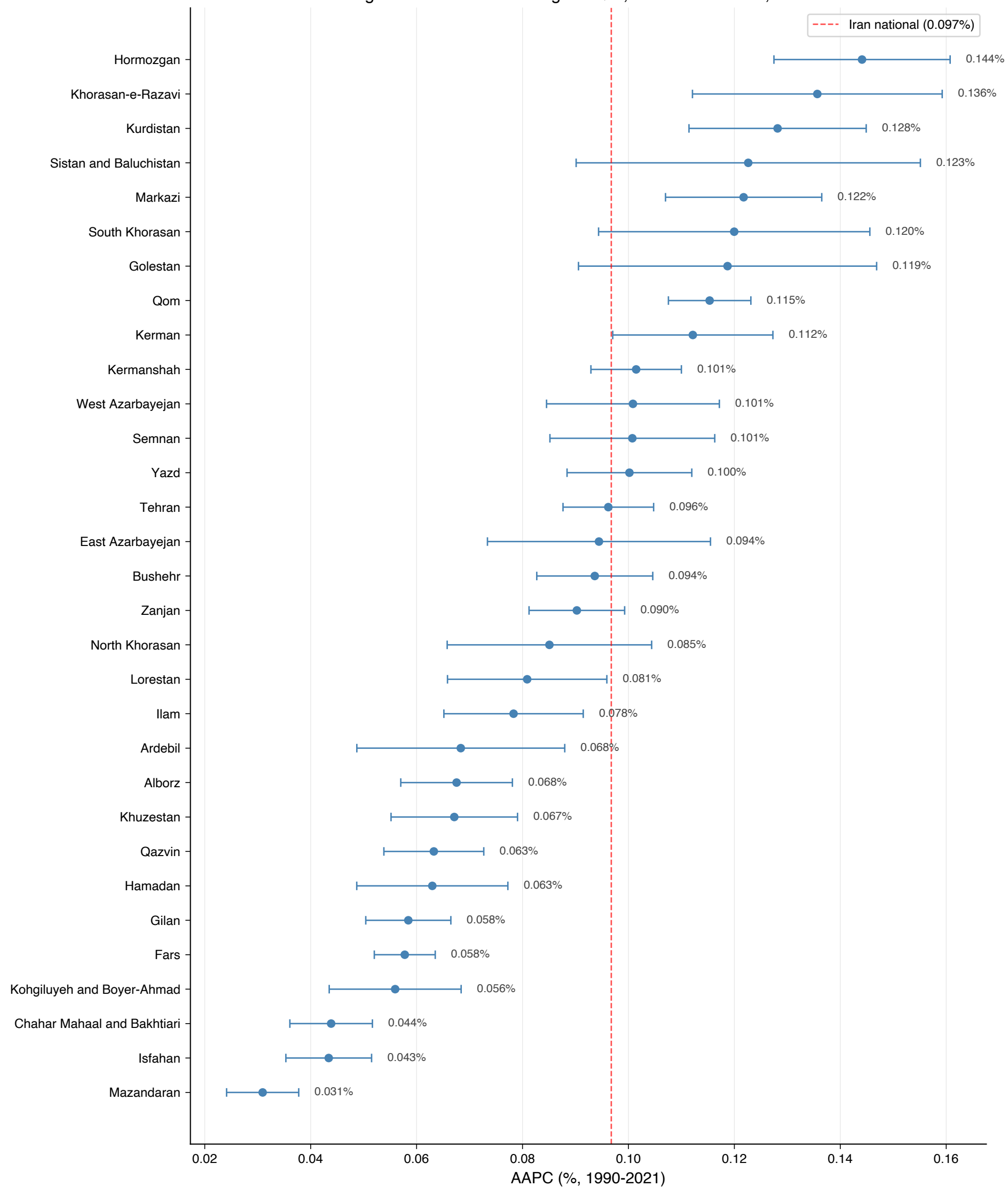
Average Annual Percent Change in QCI, Iranian Provinces, 1990-2021
