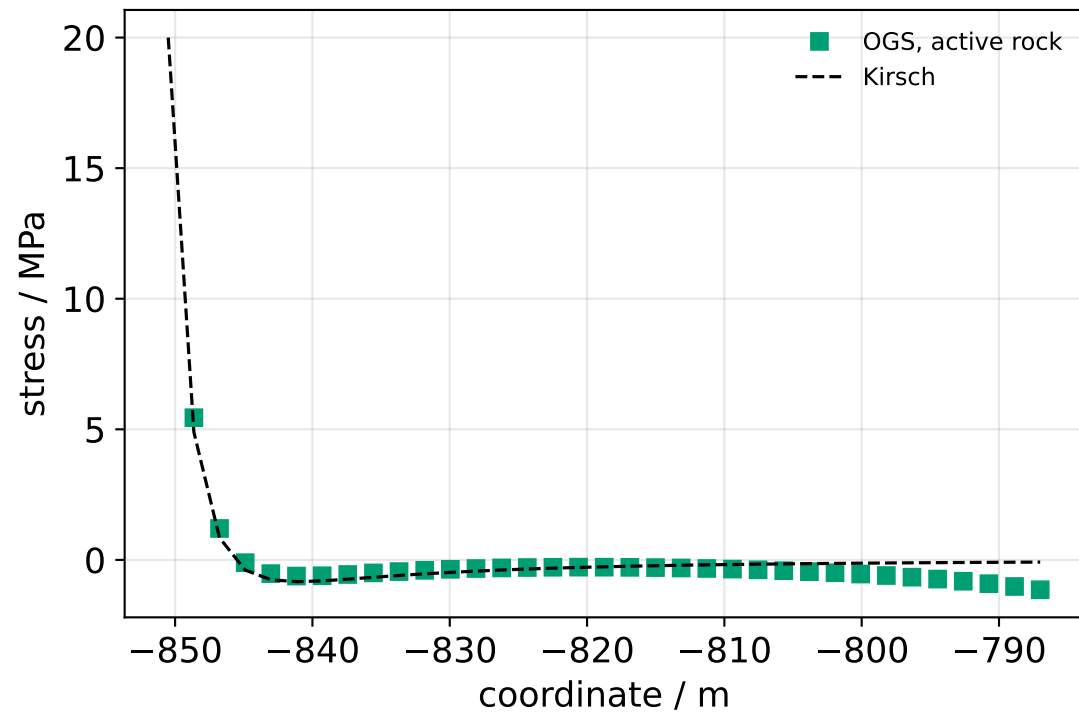
\sigma_{\theta\theta}, \theta = 90^\circ
