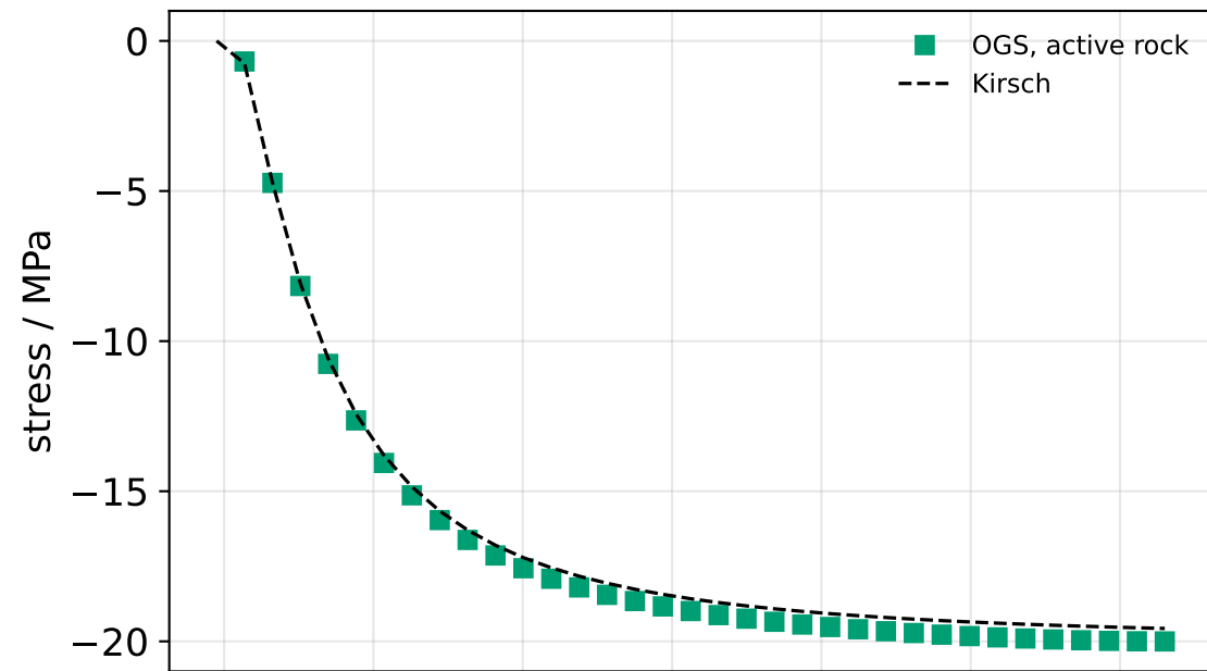
\sigma_{rr}, \theta = 90^\circ
