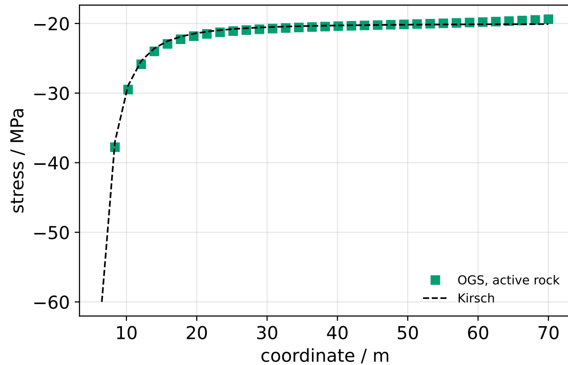
\sigma_{\theta\theta}, \theta = 0^\circ
