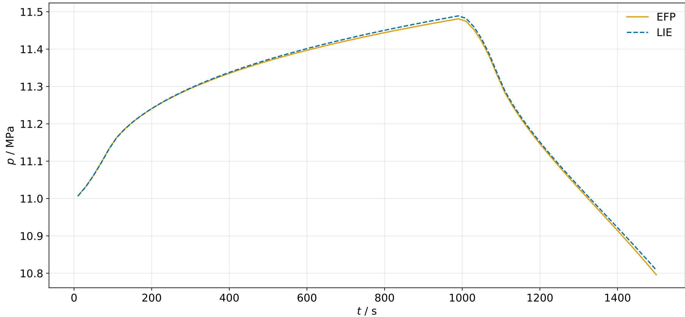
Pressure over Time at Inlet
