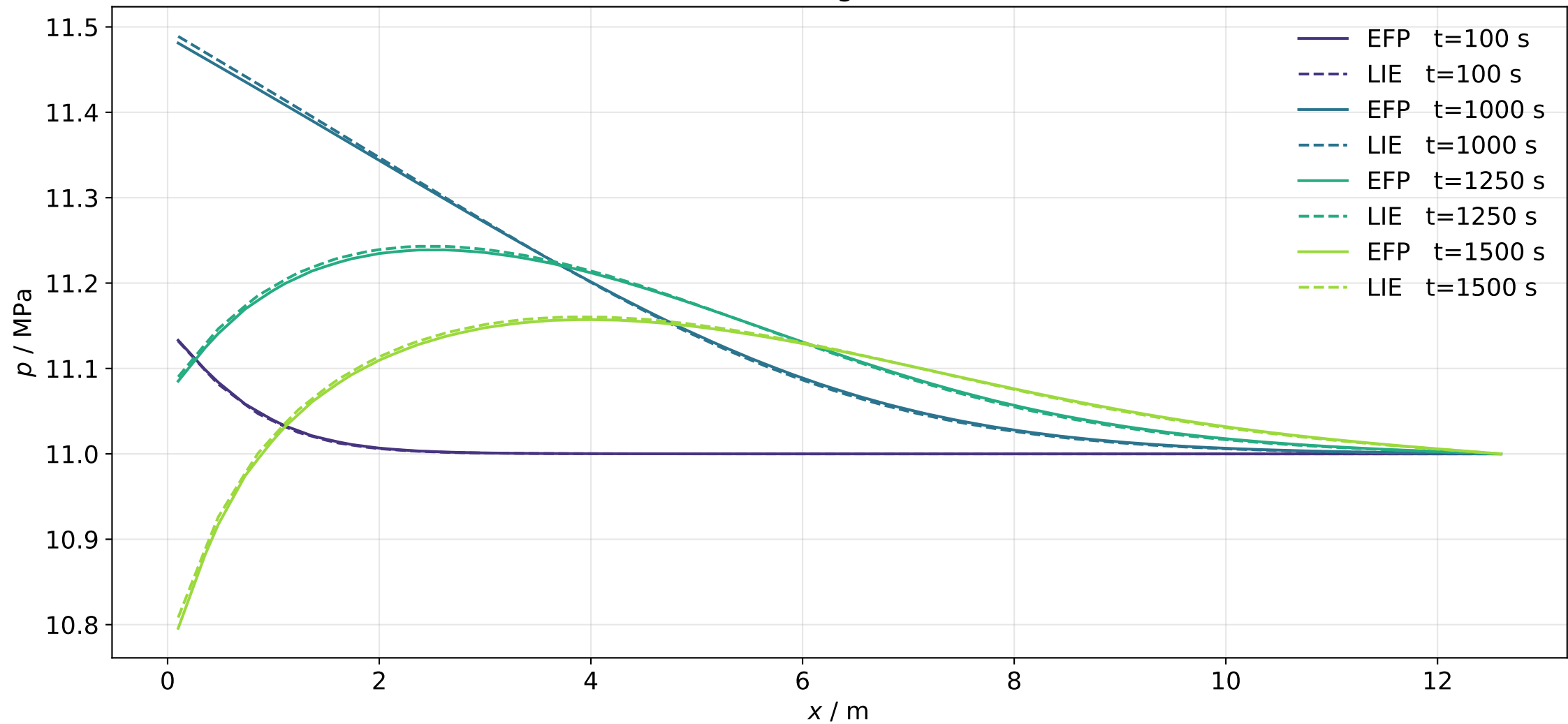
Pressure Along the Fracture
