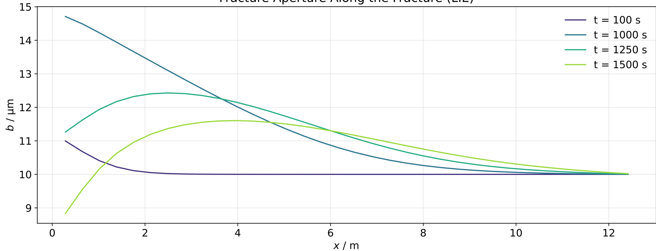
Fracture Aperture Along the Fracture (LIE)
