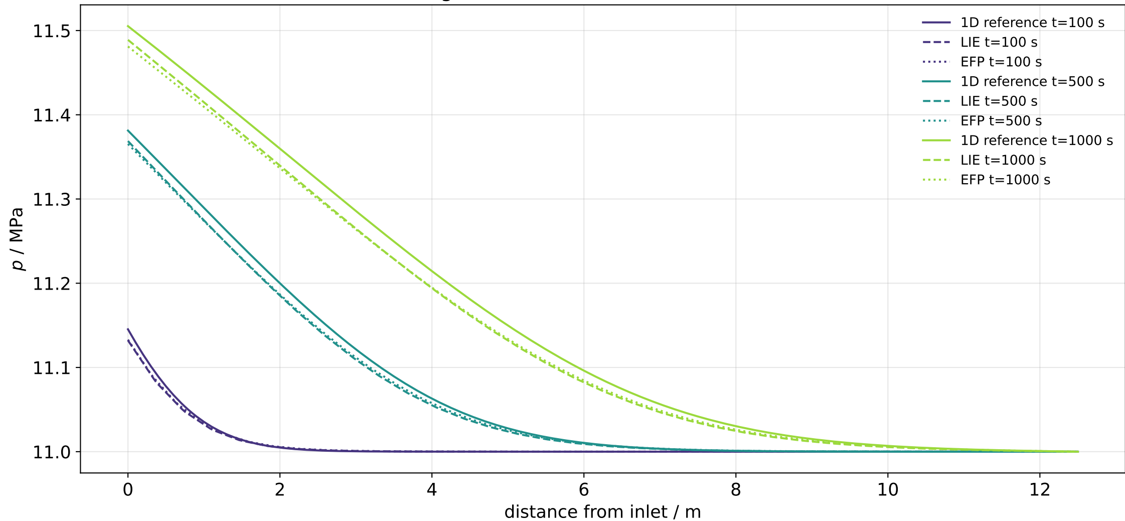
Pressure Along the Fracture: Simulations vs. 1D Reference
