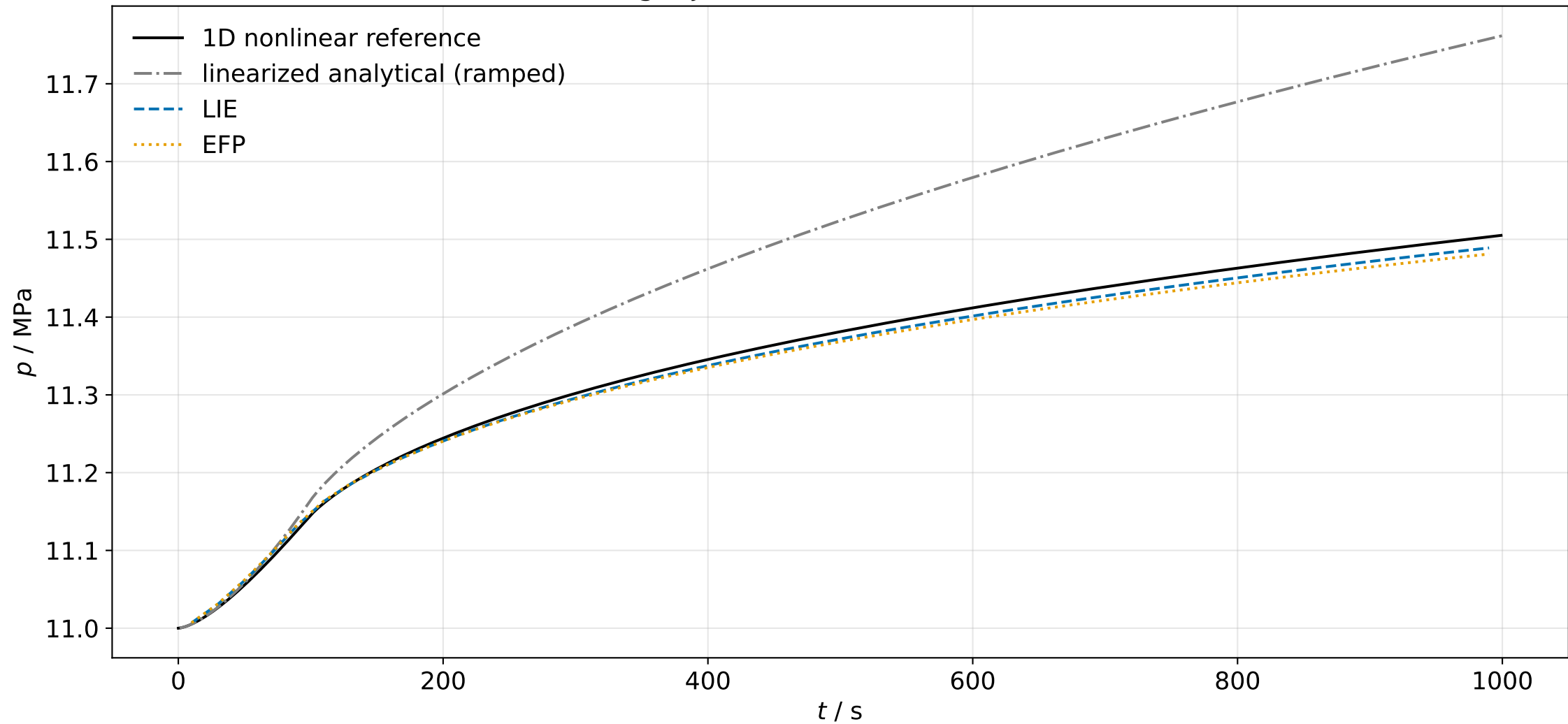
Inlet Pressure During Injection: Simulations vs. Reference Solutions
